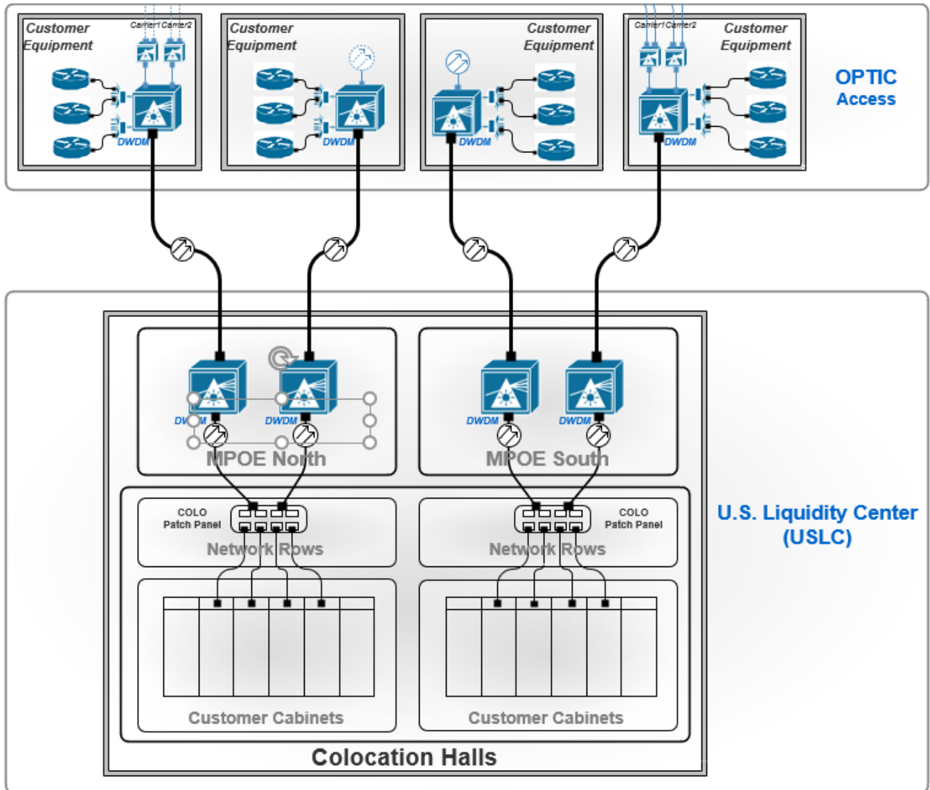
(Figure 9) – IGN Optic
