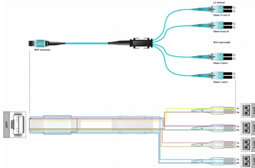
(Figure 12) - Example - Fan Out Cable
